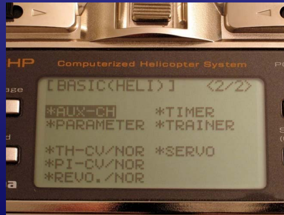
Futaba T9CHP transmitter: Primary screen showing select model (HawkPro), digital trims and timers (left); basic programming menu (middle); advanced programming menu (right) (Photos by W. Witt)
